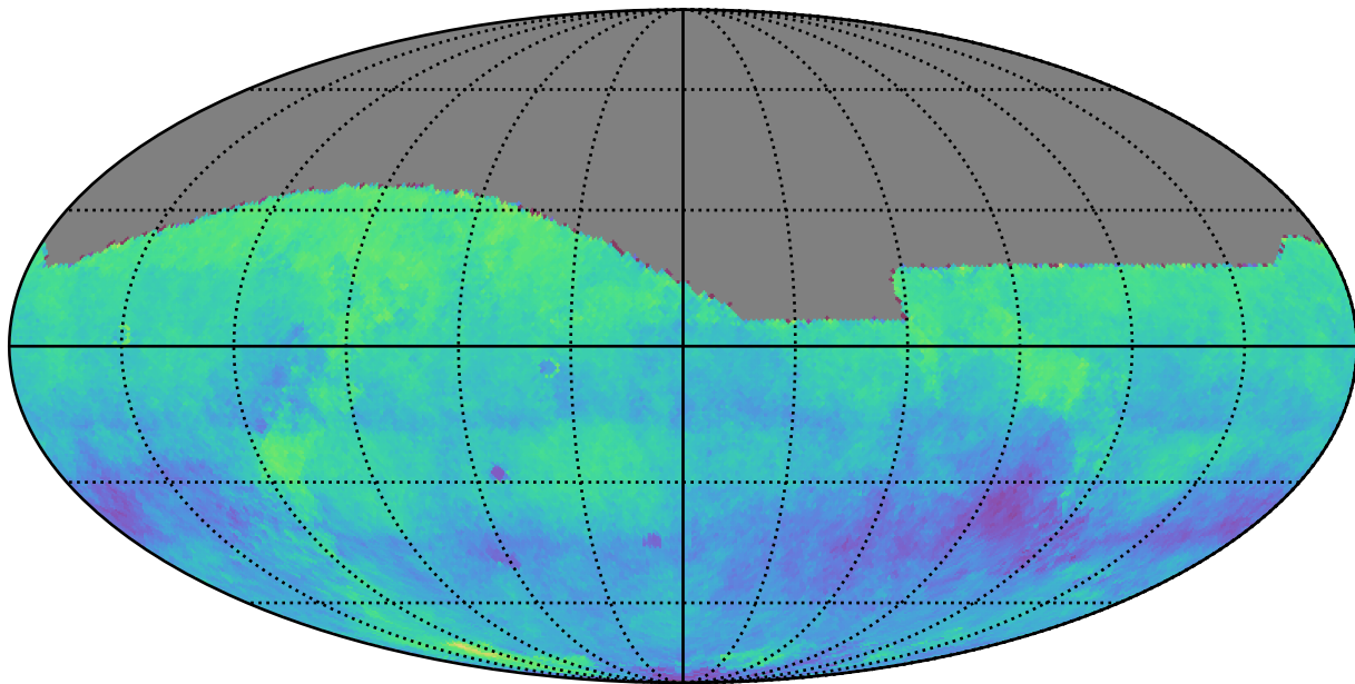
roll_pause_mjdp0_v3.4_10yrs i: Kuiper rotSkyPos
