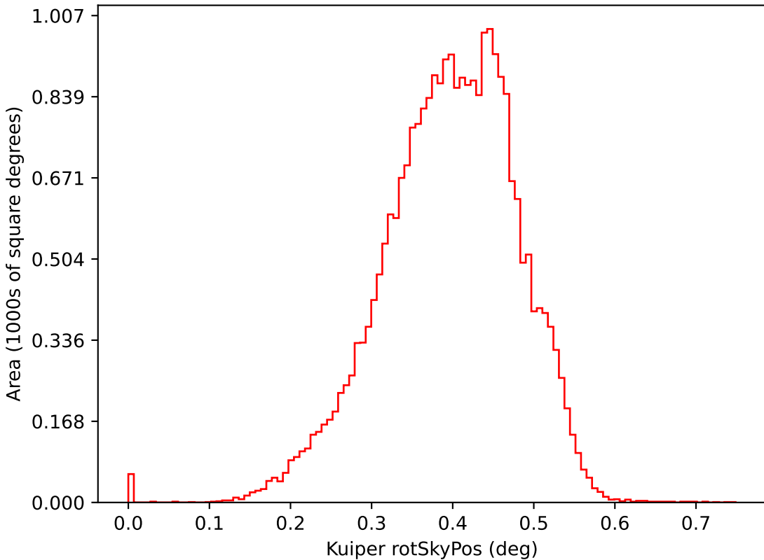
roll_pause_mjdp0_v3.4_10yrs i: Kuiper rotSkyPos
