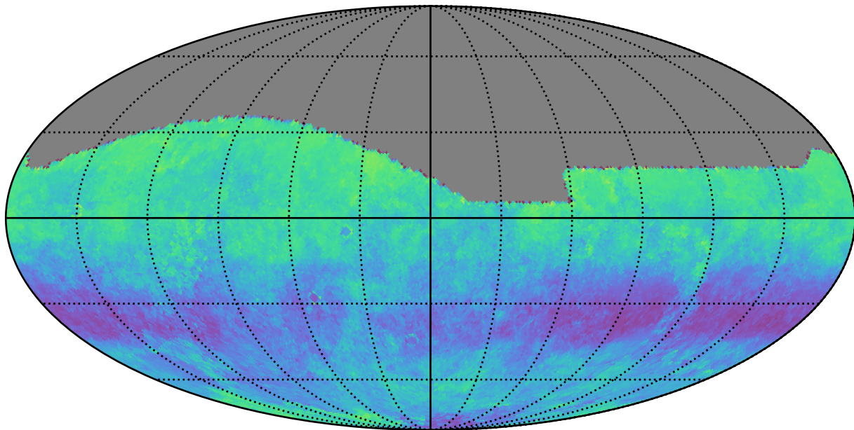
roll_pause_mjdp0_v3.4_10yrs g: Kuiper rotSkyPos
