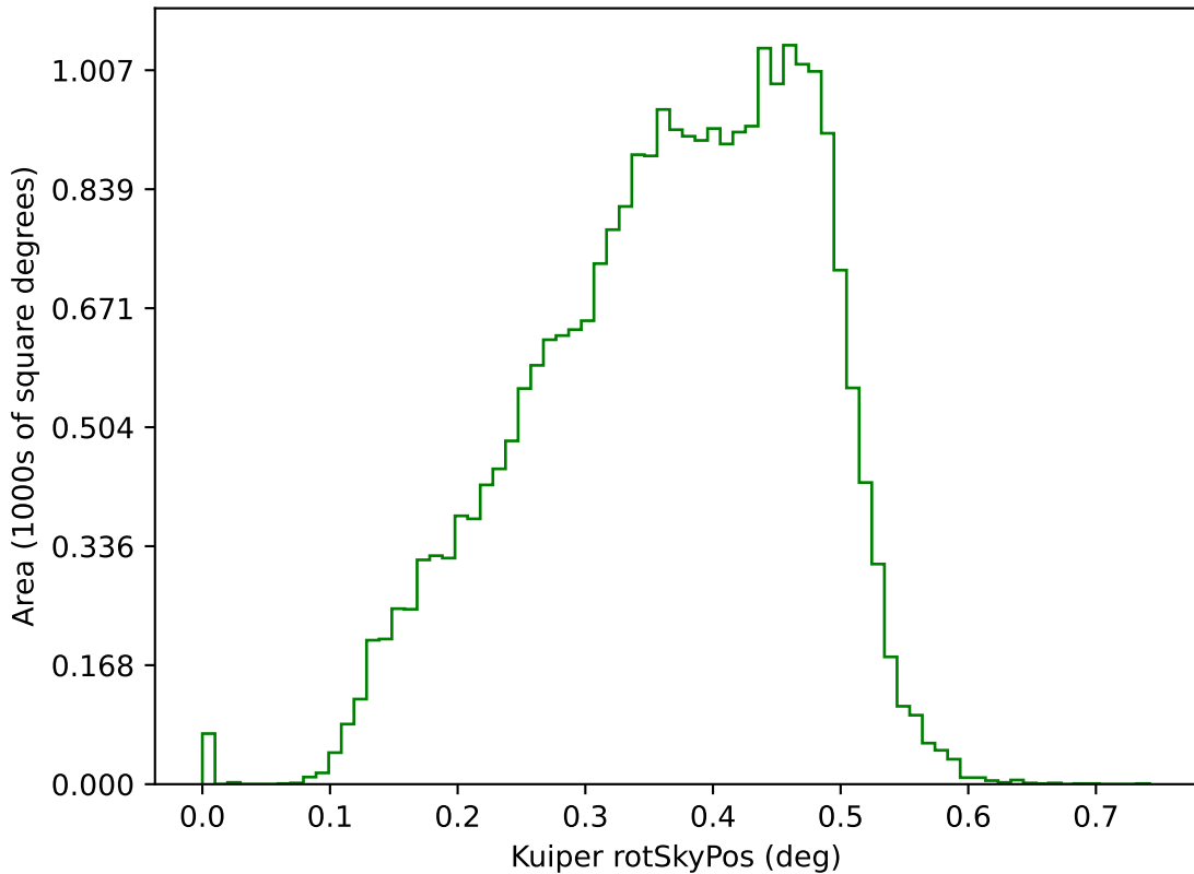
roll_pause_mjdp0_v3.4_10yrs g: Kuiper rotSkyPos
