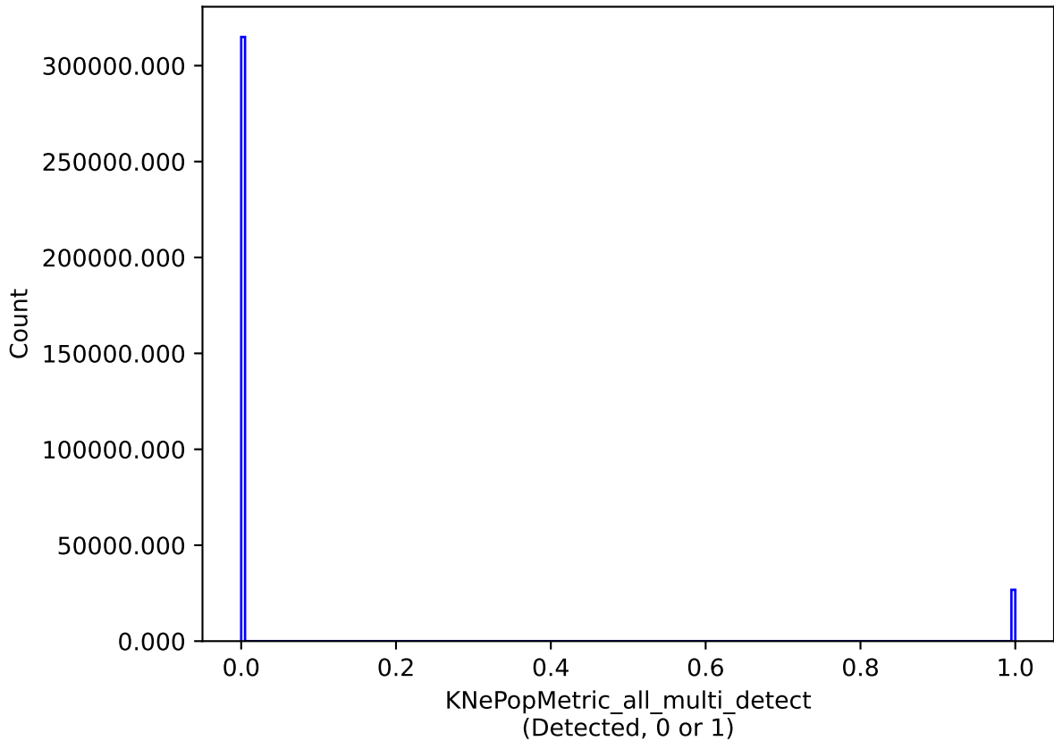
roll_pause_mjdp0_v3.4_10yrs all models: KNePopMetric_all_multi_detect
