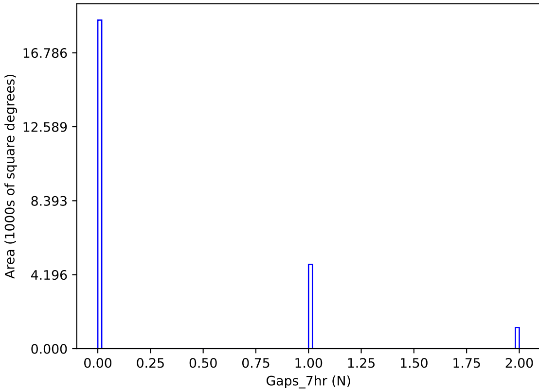
roll_pause_mjdp0_v3.4_10yrs y band: Gaps_7hr
