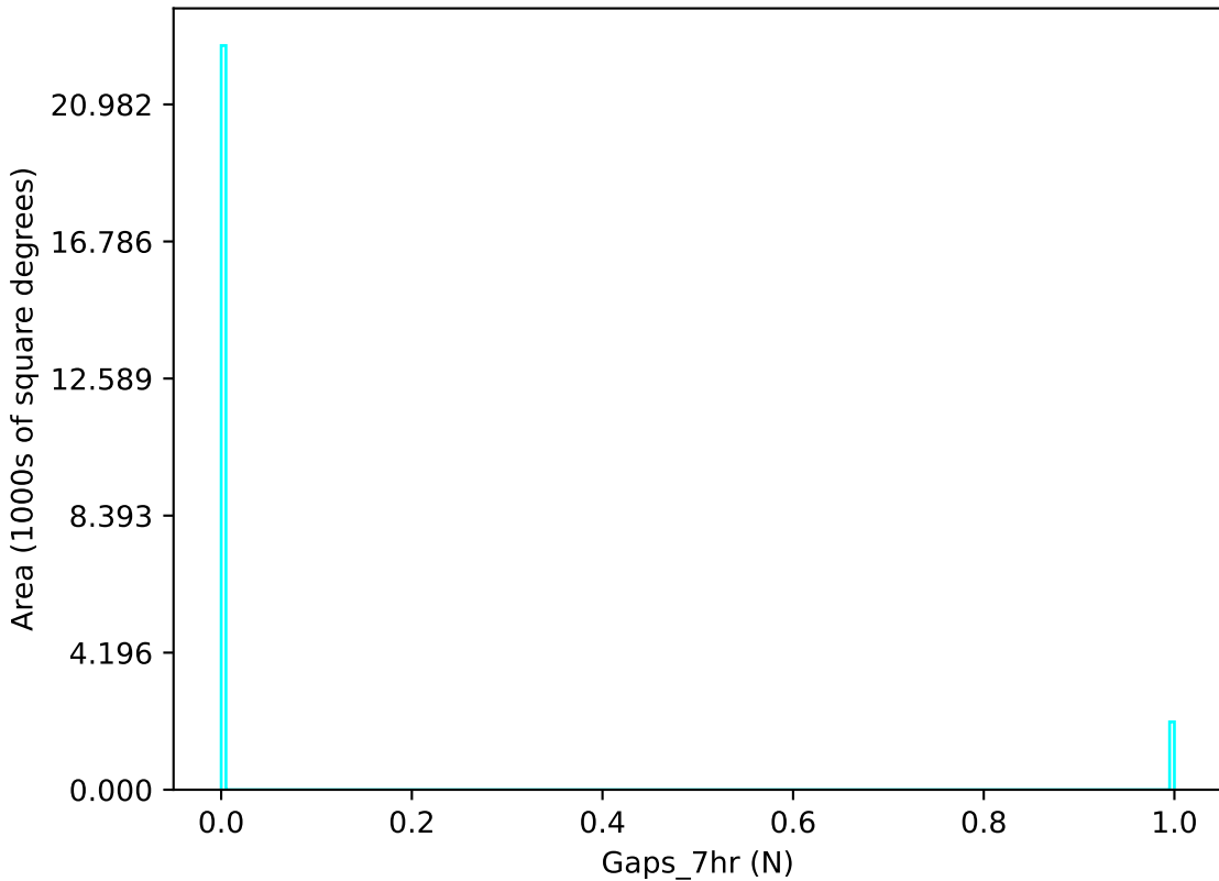
roll_pause_mjdp0_v3.4_10yrs u band: Gaps_7hr
