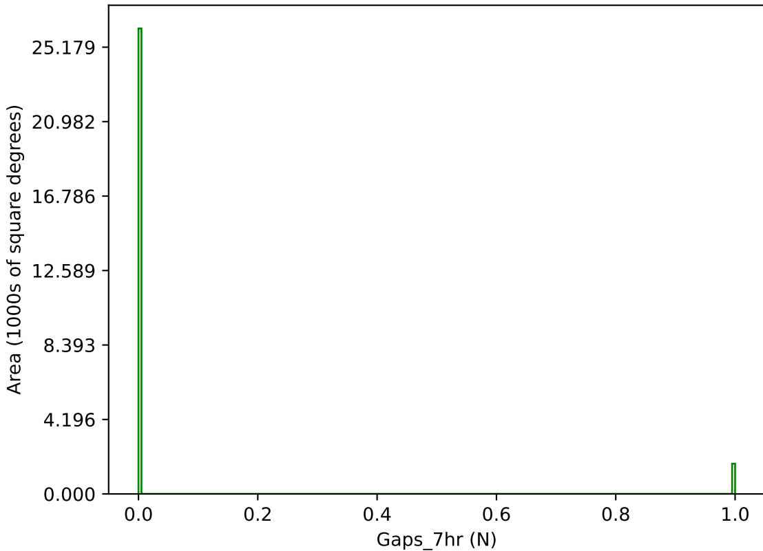
roll_pause_mjdp0_v3.4_10yrs g band: Gaps_7hr
