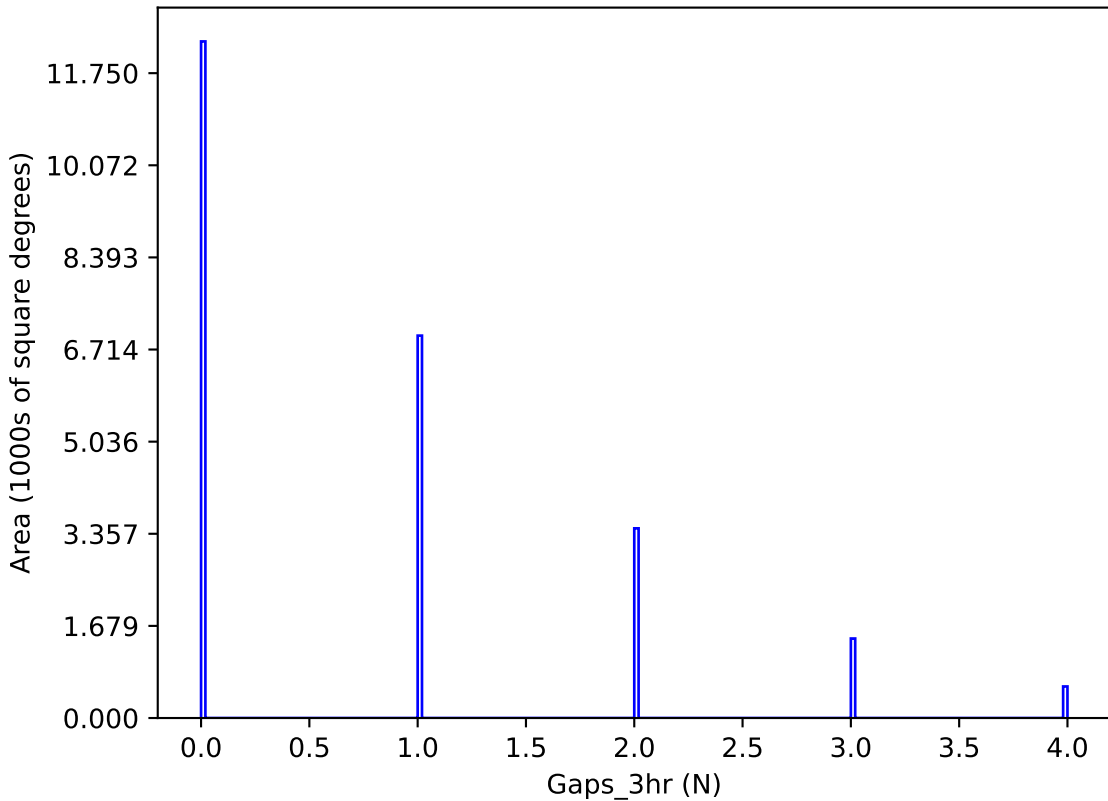
roll_pause_mjdp0_v3.4_10yrs y band: Gaps_3hr
