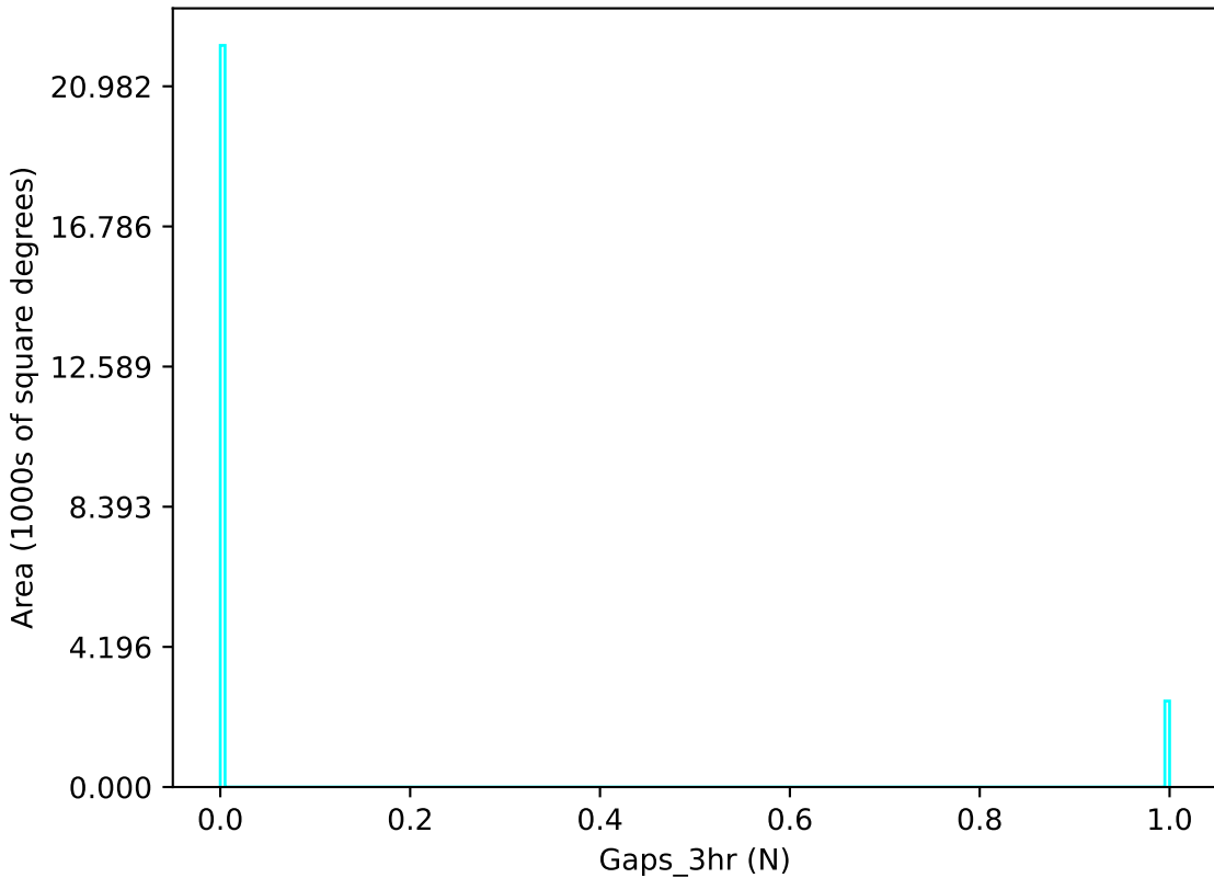
roll_pause_mjdp0_v3.4_10yrs u band: Gaps_3hr
