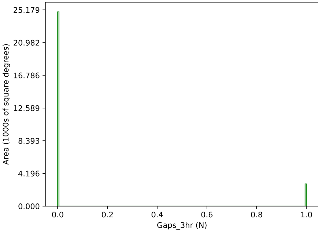
roll_pause_mjdp0_v3.4_10yrs g band: Gaps_3hr
