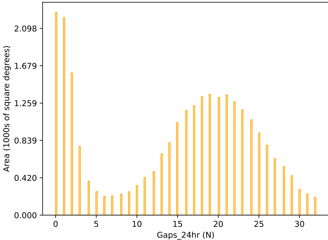
roll_pause_mjdp0_v3.4_10yrs r band: Gaps_24hr
