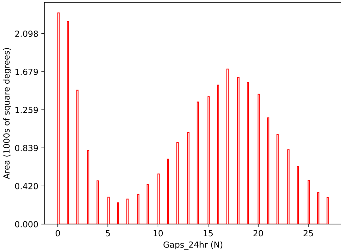
roll_pause_mjdp0_v3.4_10yrs i band: Gaps_24hr
