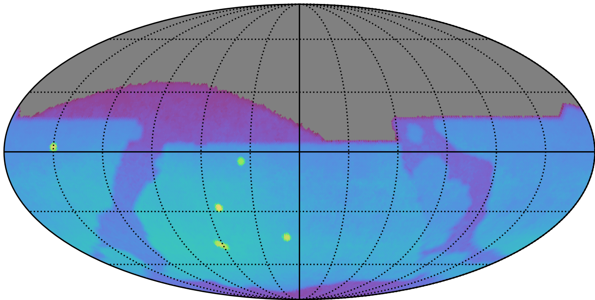
roll_pause_mjdp0_v3.4_10yrs : Brown Dwarf, L7
