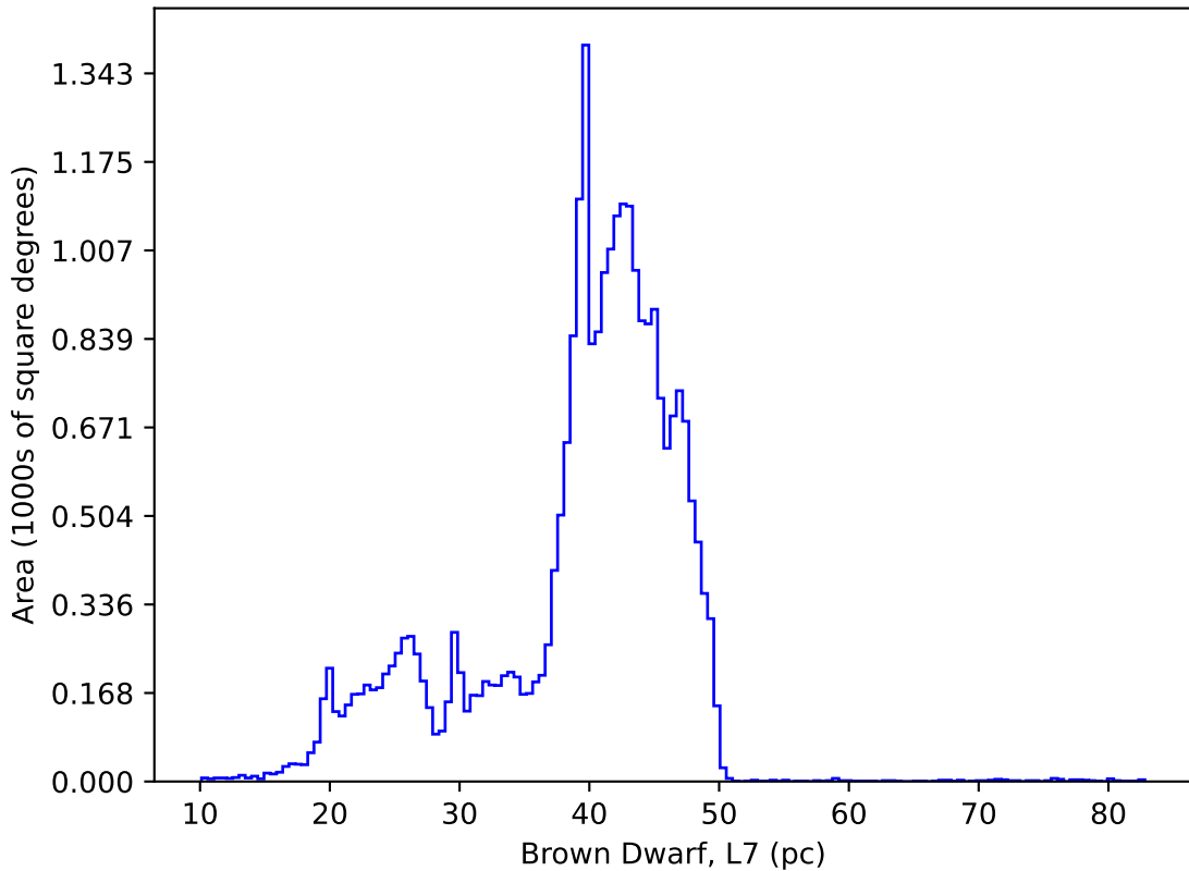
roll_pause_mjdp0_v3.4_10yrs : Brown Dwarf, L7
