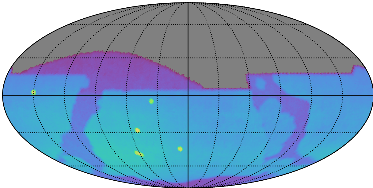
roll_pause_mjdp0_v3.4_10yrs : Brown Dwarf, L4
