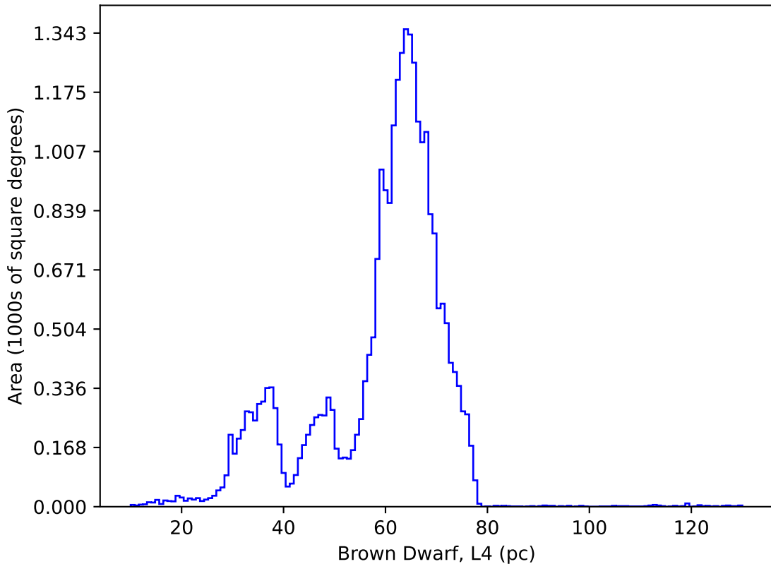
roll_pause_mjdp0_v3.4_10yrs : Brown Dwarf, L4
