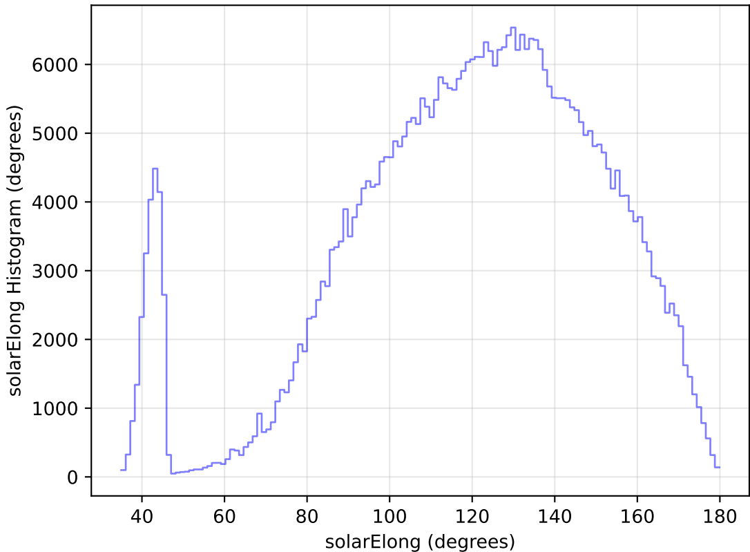
roll_pause_mjdp0_v3.4_10yrs WFD z band: solarElong Histogram
