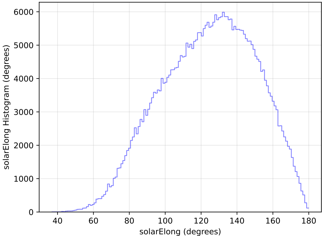
roll_pause_mjdp0_v3.4_10yrs WFD y band: solarElong Histogram
