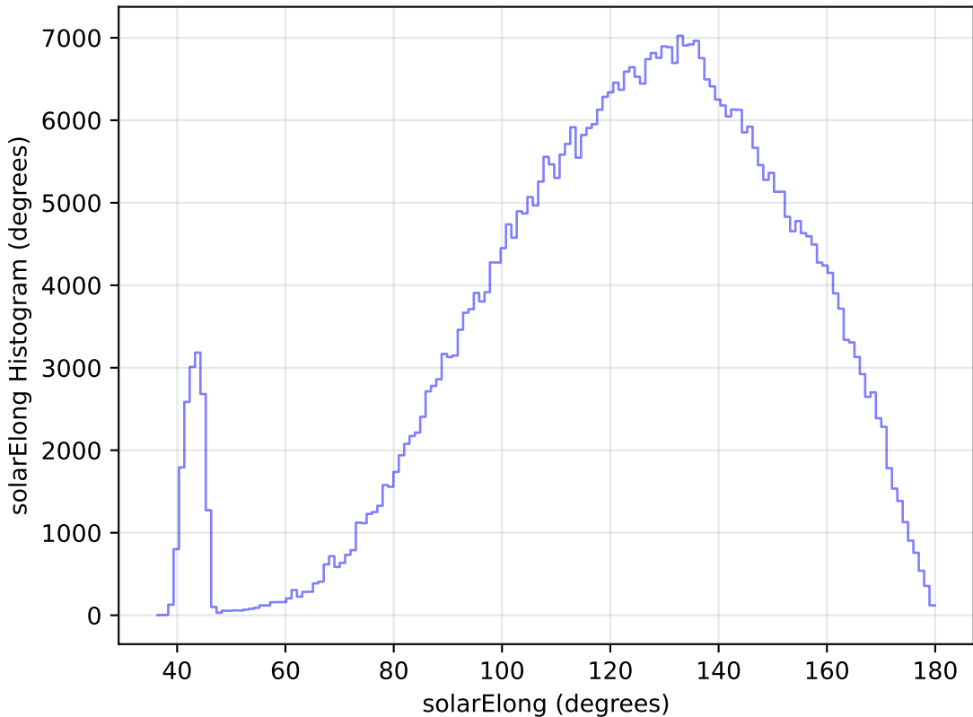
roll_pause_mjdp0_v3.4_10yrs WFD r band: solarElong Histogram
