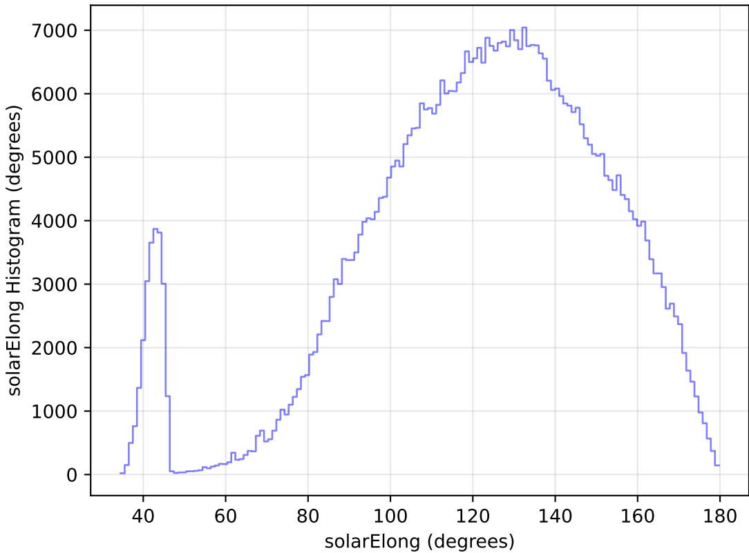
roll_pause_mjdp0_v3.4_10yrs WFD i band: solarElong Histogram
