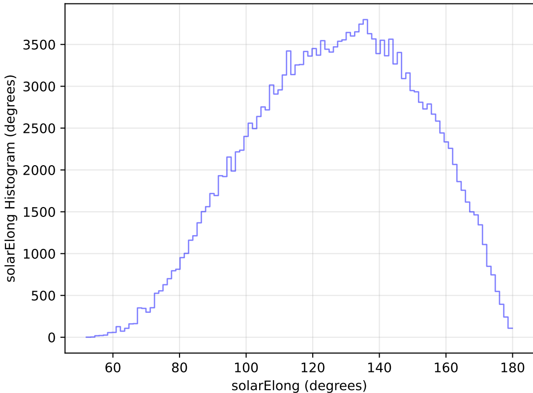
roll_pause_mjdp0_v3.4_10yrs WFD g band: solarElong Histogram
