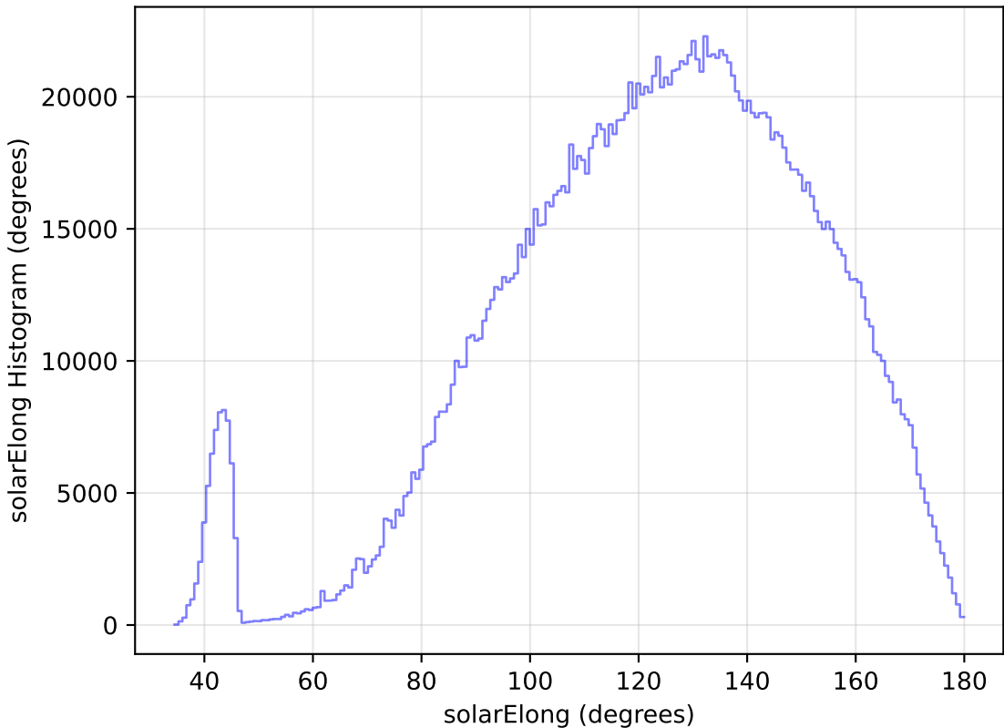
roll_pause_mjdp0_v3.4_10yrs WFD all bands: solarElong Histogram
