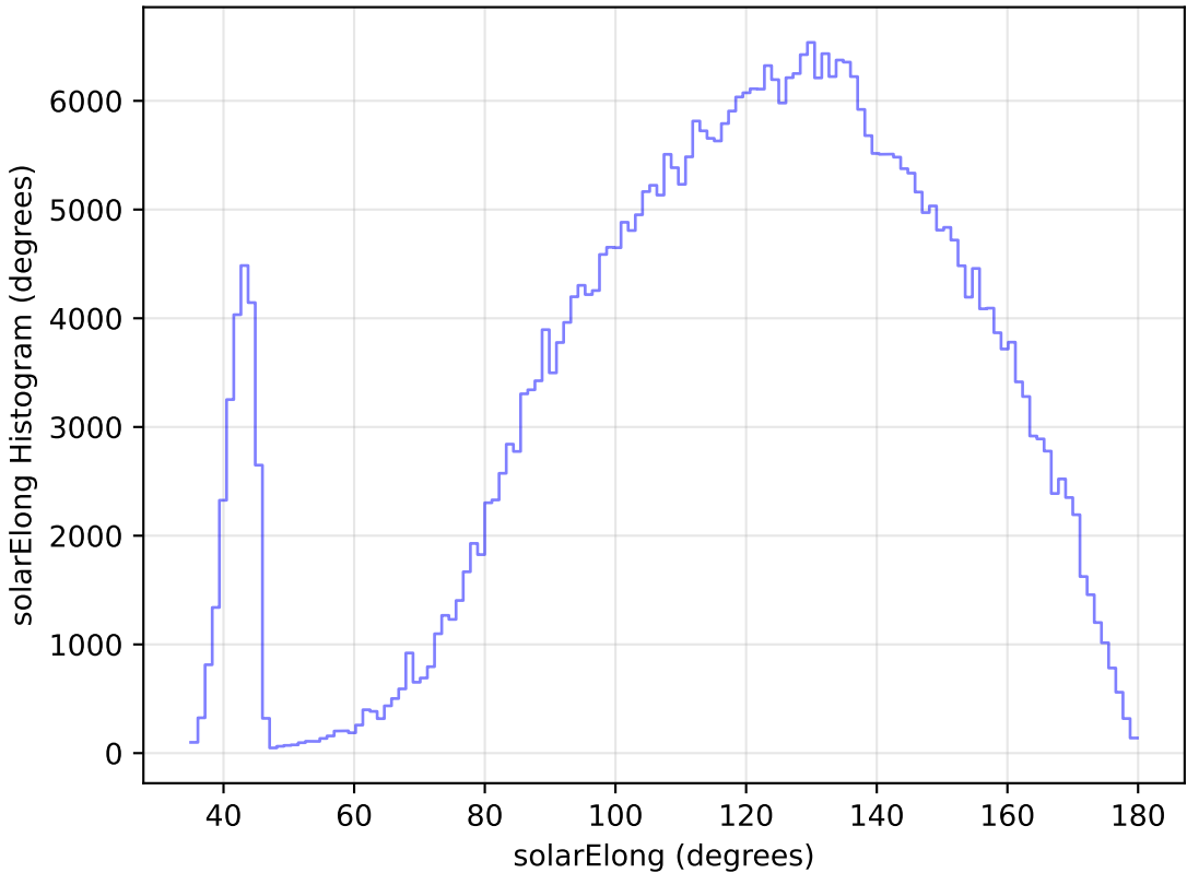
roll_pause_mjdp0_v3.4_10yrs All sky z band: solarElong Histogram
