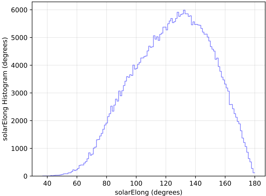
roll_pause_mjdp0_v3.4_10yrs All sky y band: solarElong Histogram
