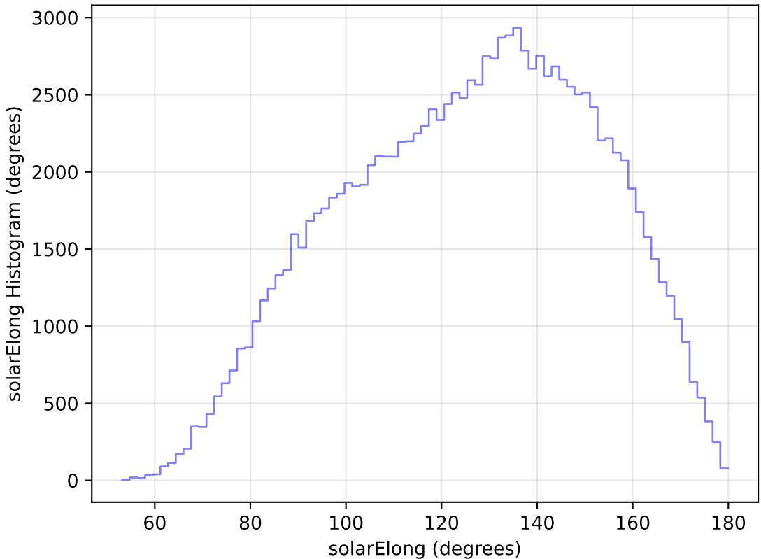
roll_pause_mjdp0_v3.4_10yrs All sky u band: solarElong Histogram
