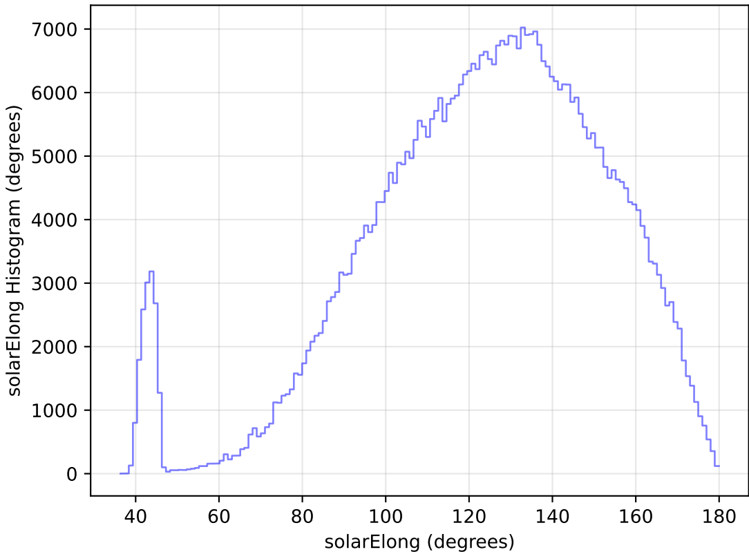
roll_pause_mjdp0_v3.4_10yrs All sky r band: solarElong Histogram
