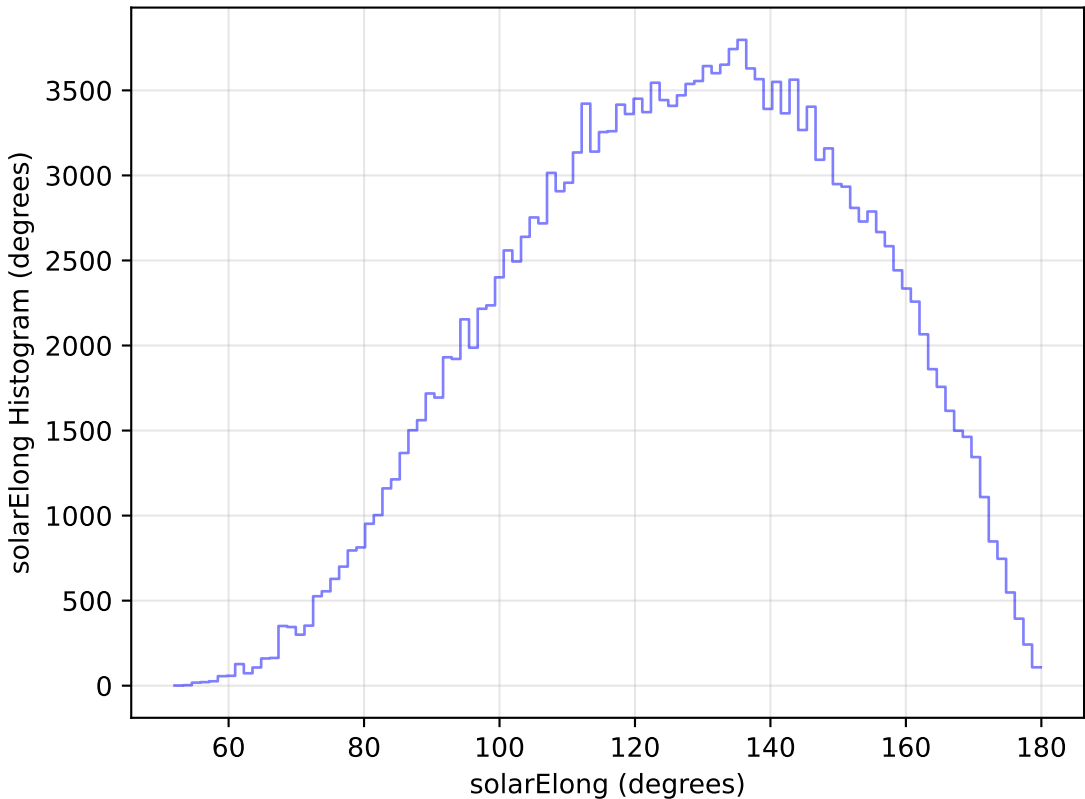
roll_pause_mjdp0_v3.4_10yrs All sky g band: solarElong Histogram
