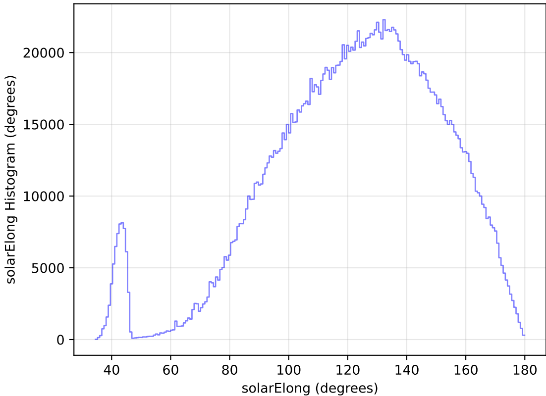
roll_pause_mjdp0_v3.4_10yrs All sky all bands: solarElong Histogram
