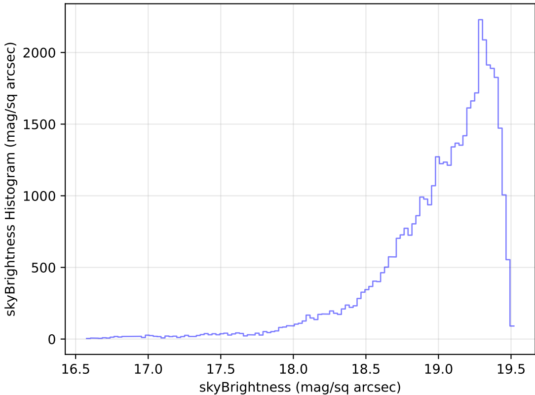
roll_pause_mjdp0_v3.4_10yrs Yr 1 z band: skyBrightness Histogram
