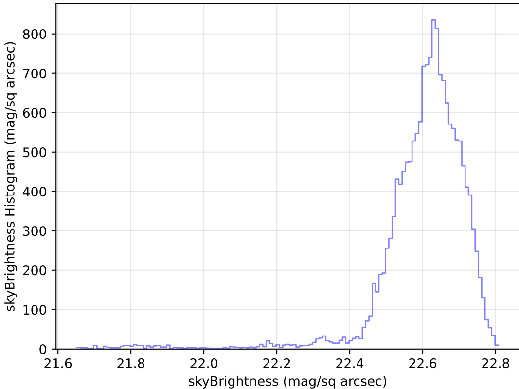
roll_pause_mjdp0_v3.4_10yrs Yr 1 u band: skyBrightness Histogram
