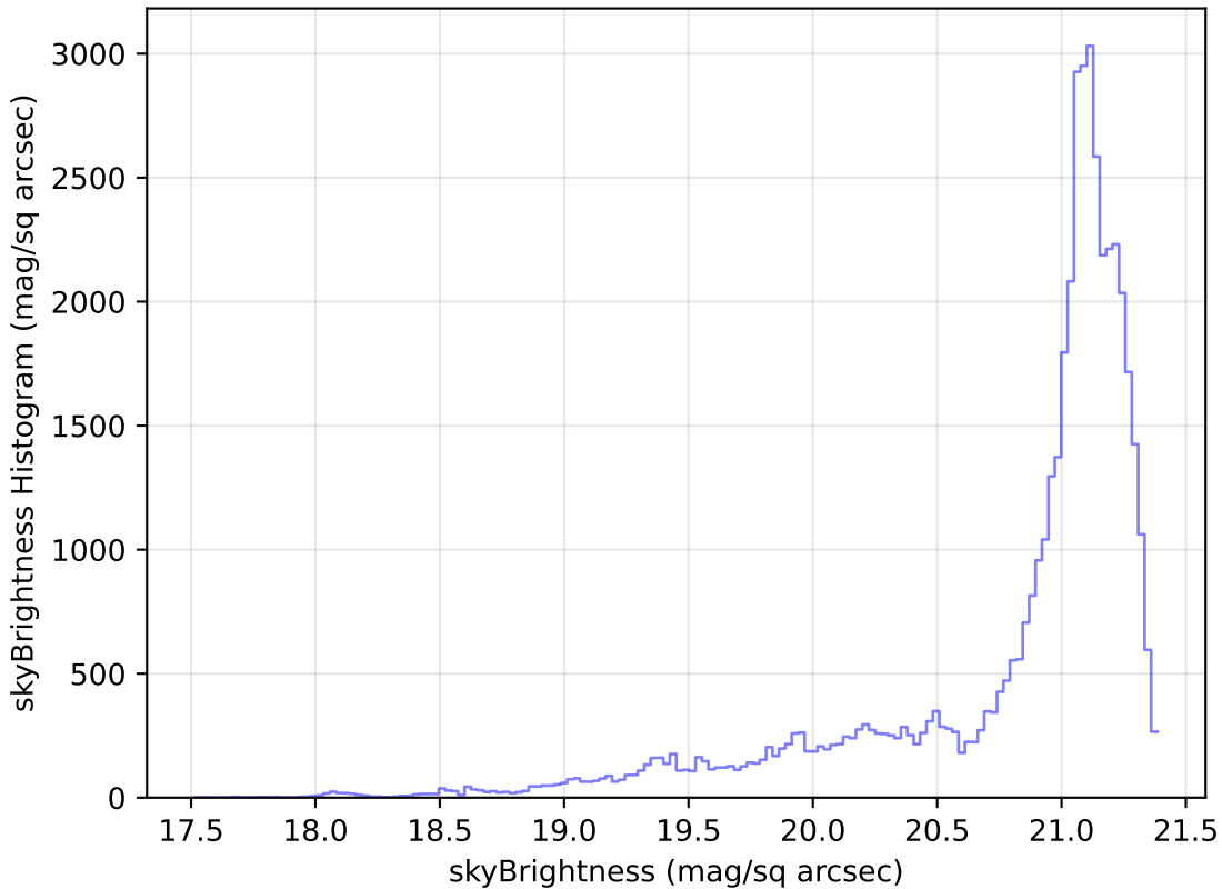
roll_pause_mjdp0_v3.4_10yrs Yr 1 r band: skyBrightness Histogram
