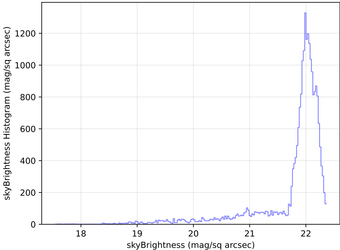
roll_pause_mjdp0_v3.4_10yrs Yr 1 g band: skyBrightness Histogram
