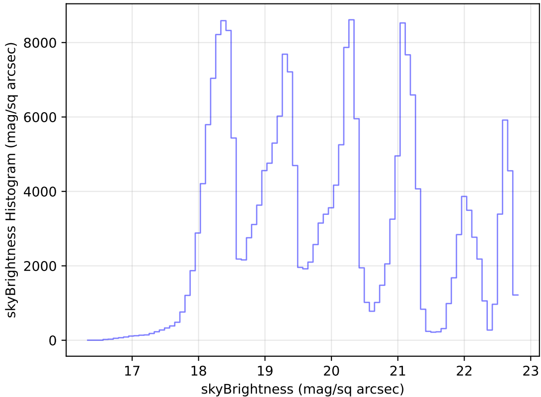
roll_pause_mjdp0_v3.4_10yrs Yr 1 all bands: skyBrightness Histogram
