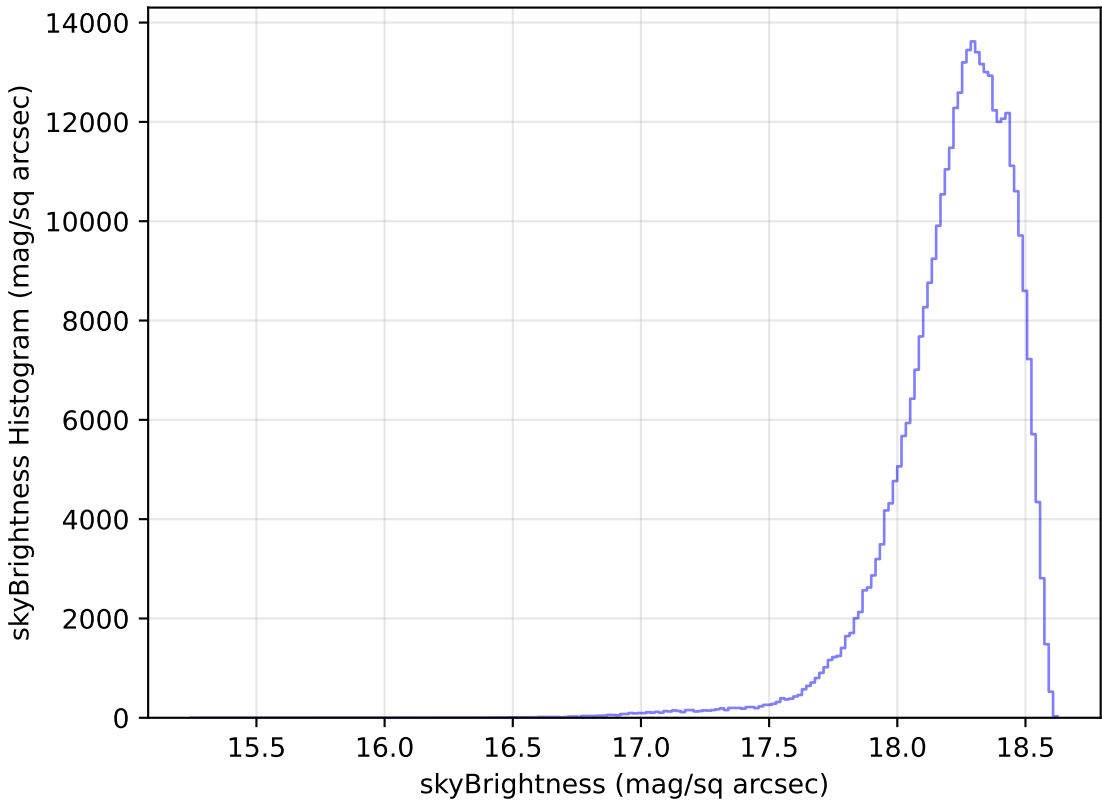
roll_pause_mjdp0_v3.4_10yrs WFD y band: skyBrightness Histogram
