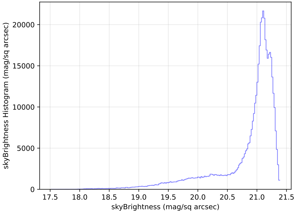
roll_pause_mjdp0_v3.4_10yrs WFD r band: skyBrightness Histogram
