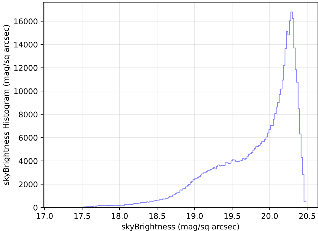
roll_pause_mjdp0_v3.4_10yrs WFD i band: skyBrightness Histogram
