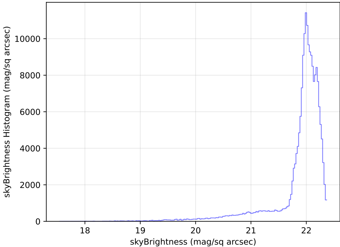
roll_pause_mjdp0_v3.4_10yrs WFD g band: skyBrightness Histogram
