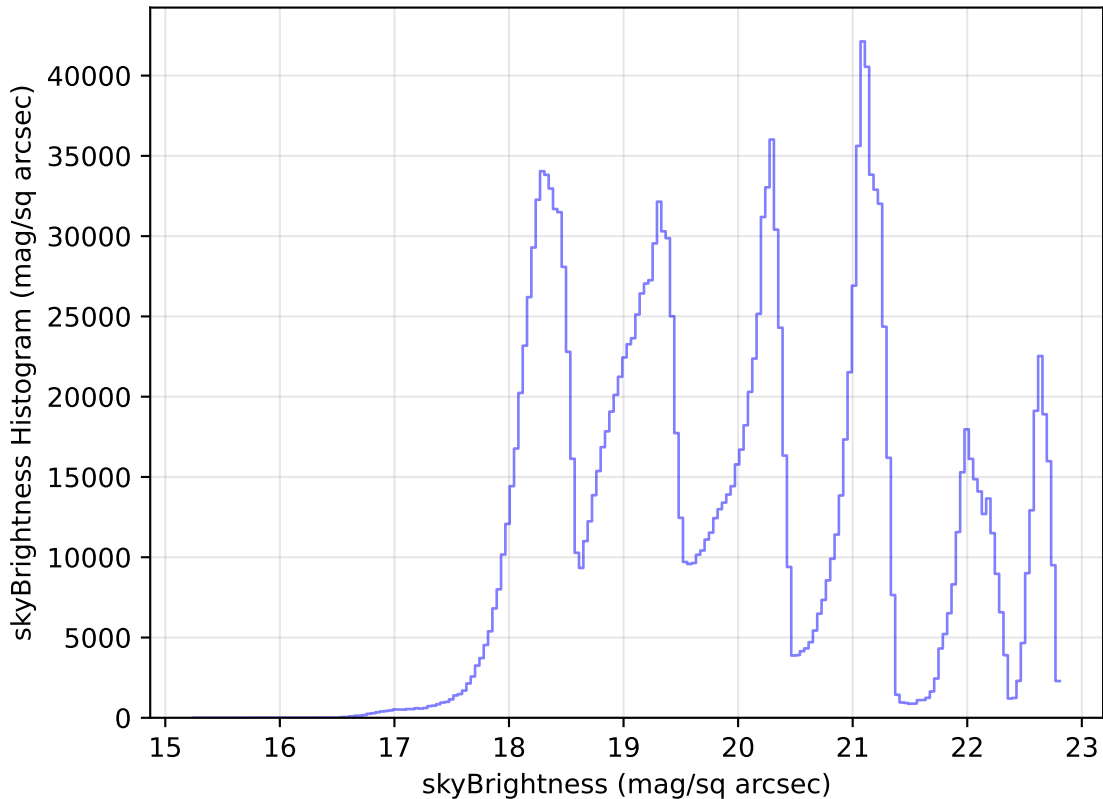
roll_pause_mjdp0_v3.4_10yrs WFD all bands: skyBrightness Histogram
