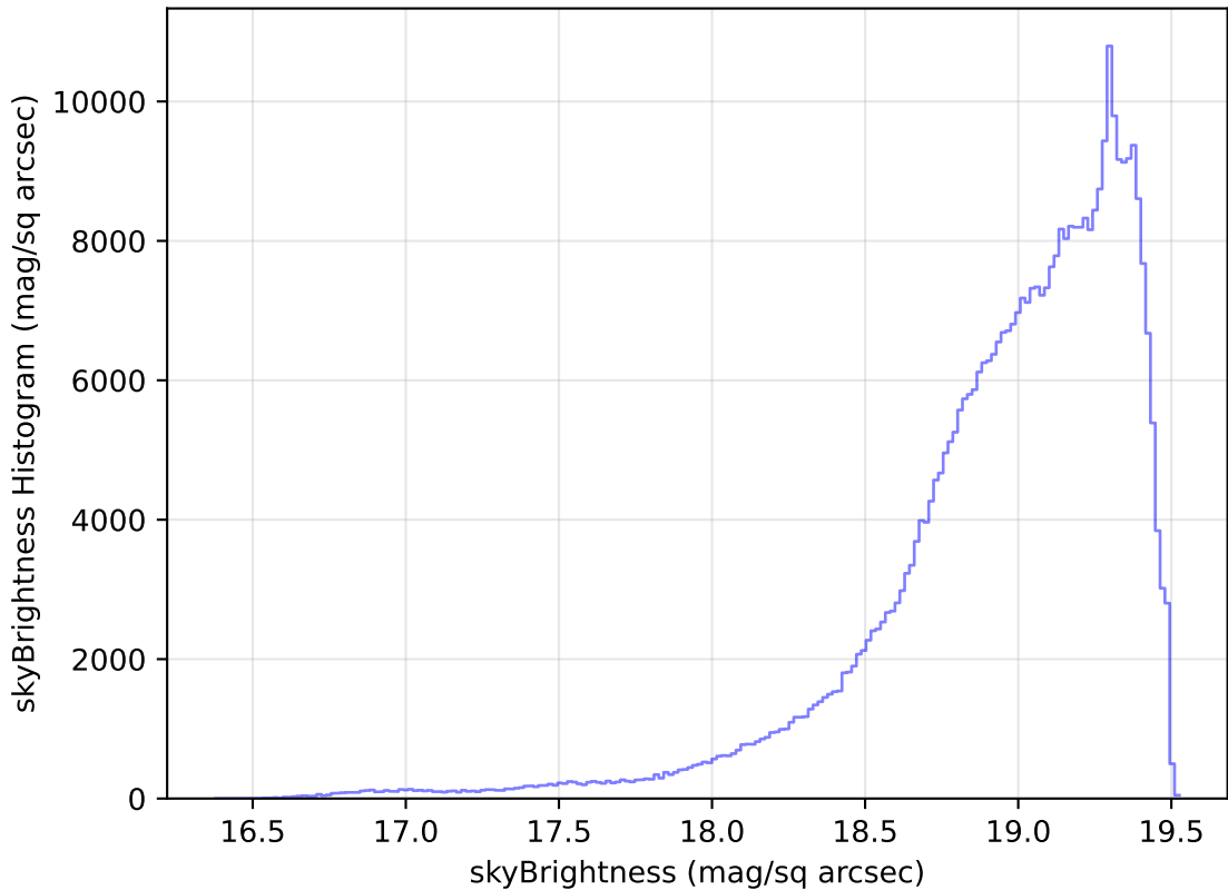
roll_pause_mjdp0_v3.4_10yrs All sky z band: skyBrightness Histogram
