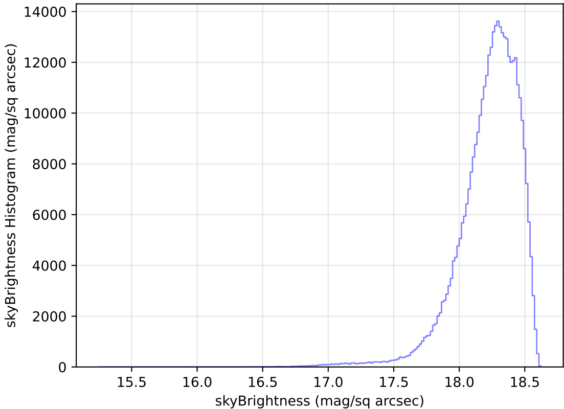
roll_pause_mjdp0_v3.4_10yrs All sky y band: skyBrightness Histogram
