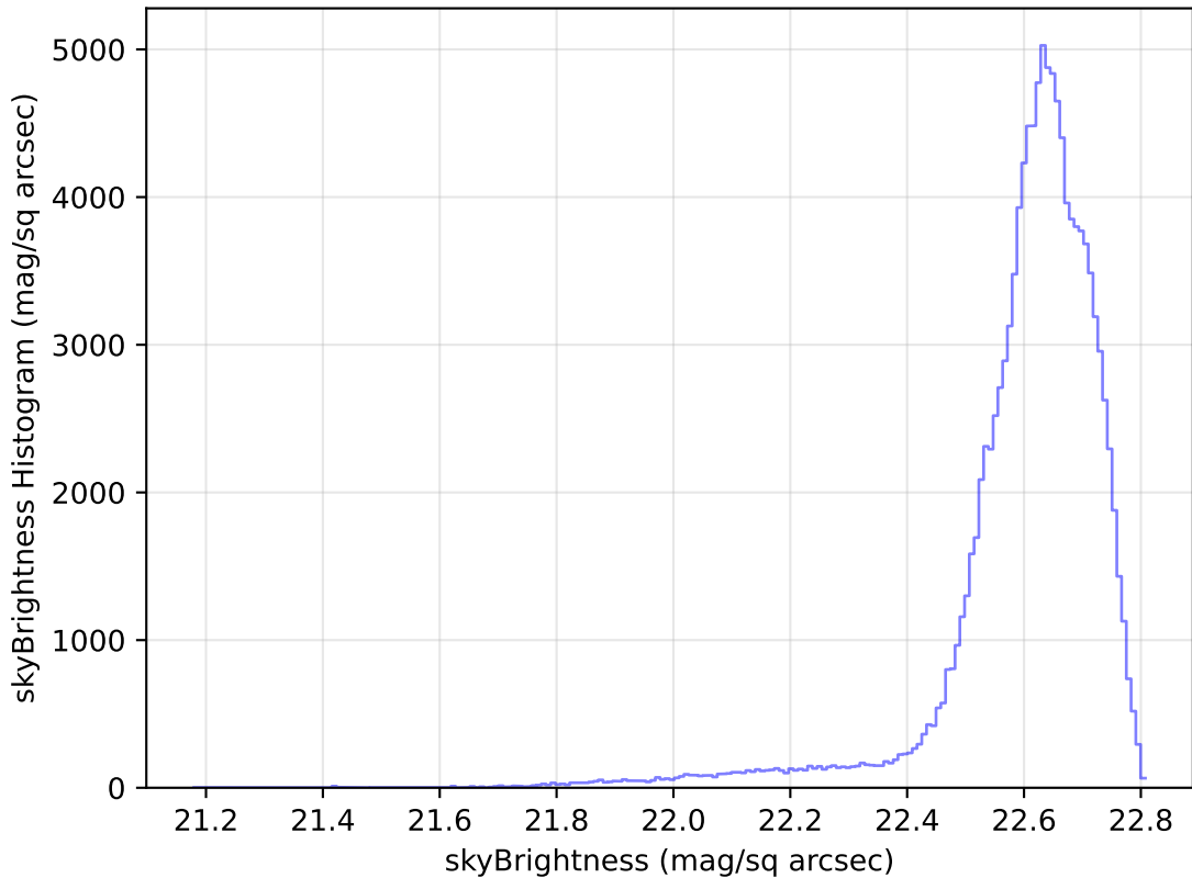
roll_pause_mjdp0_v3.4_10yrs All sky u band: skyBrightness Histogram
