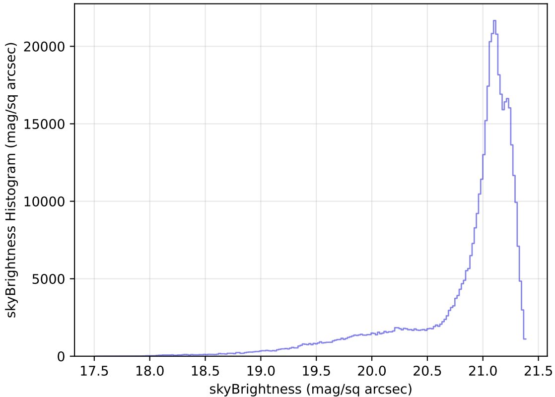
roll_pause_mjdp0_v3.4_10yrs All sky r band: skyBrightness Histogram
