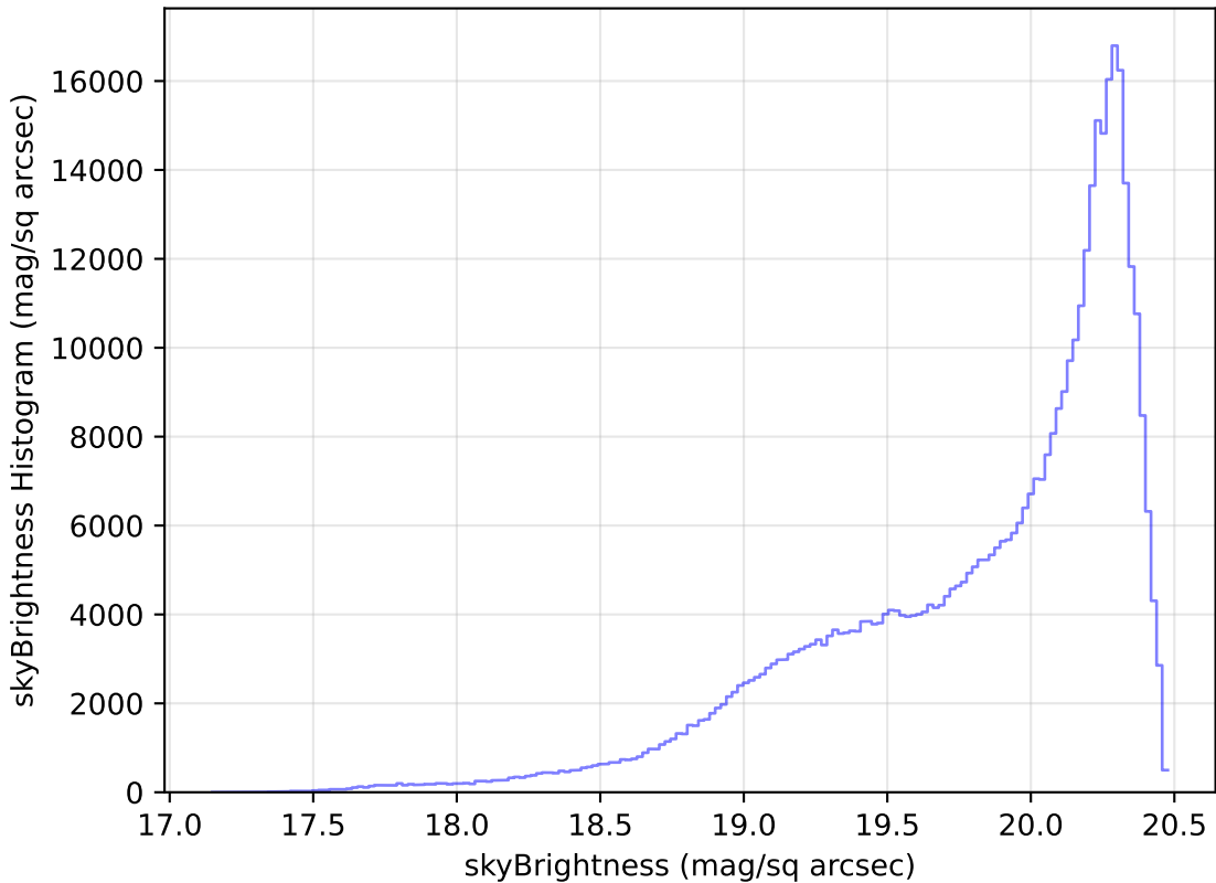
roll_pause_mjdp0_v3.4_10yrs All sky i band: skyBrightness Histogram
