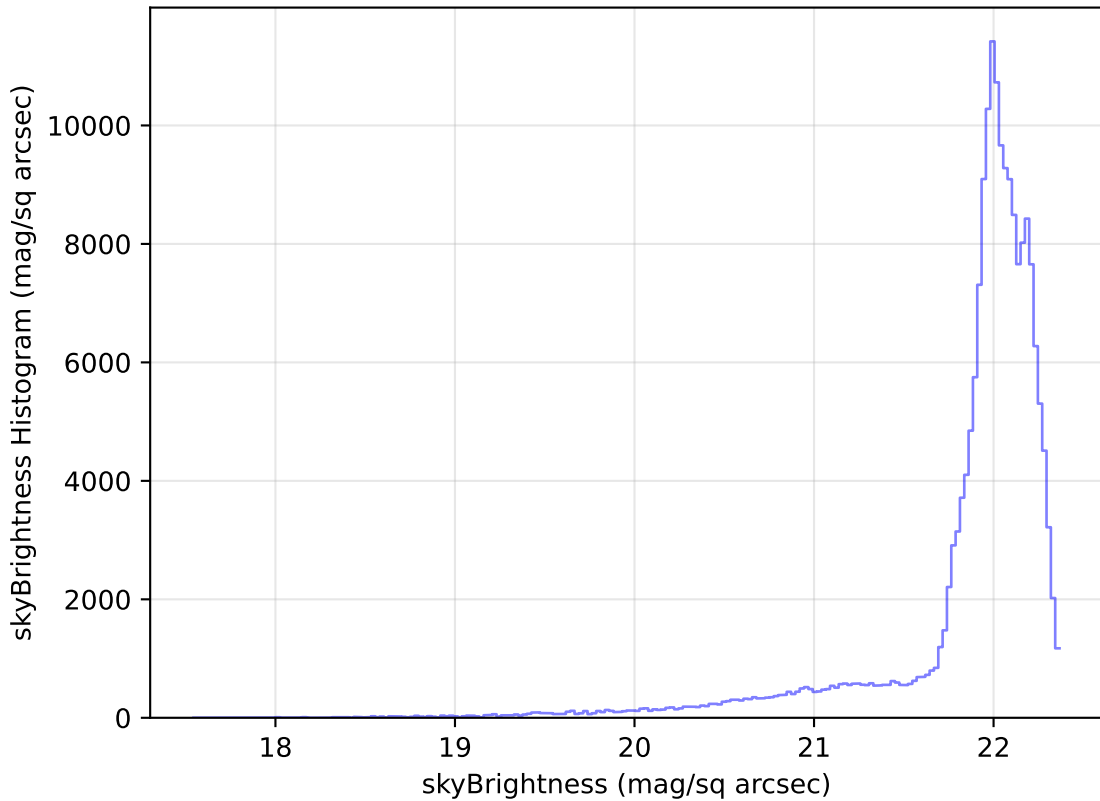
roll_pause_mjdp0_v3.4_10yrs All sky g band: skyBrightness Histogram
