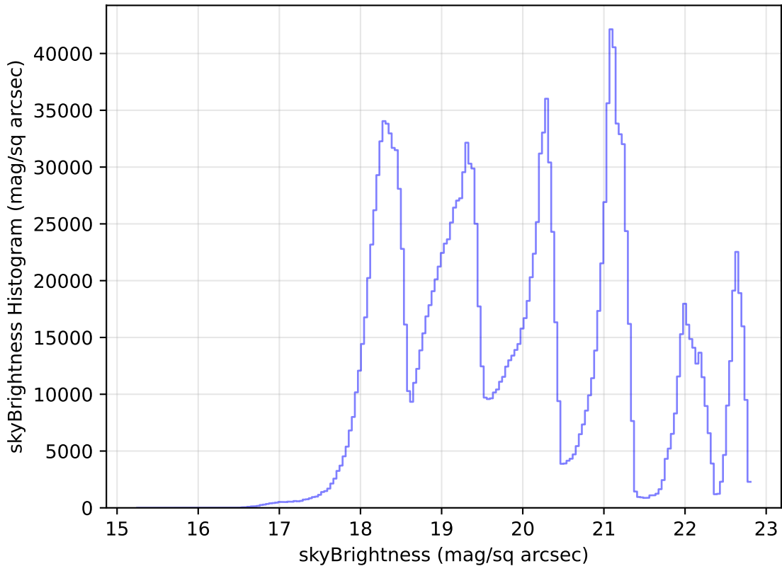
roll_pause_mjdp0_v3.4_10yrs All sky all bands: skyBrightness Histogram
