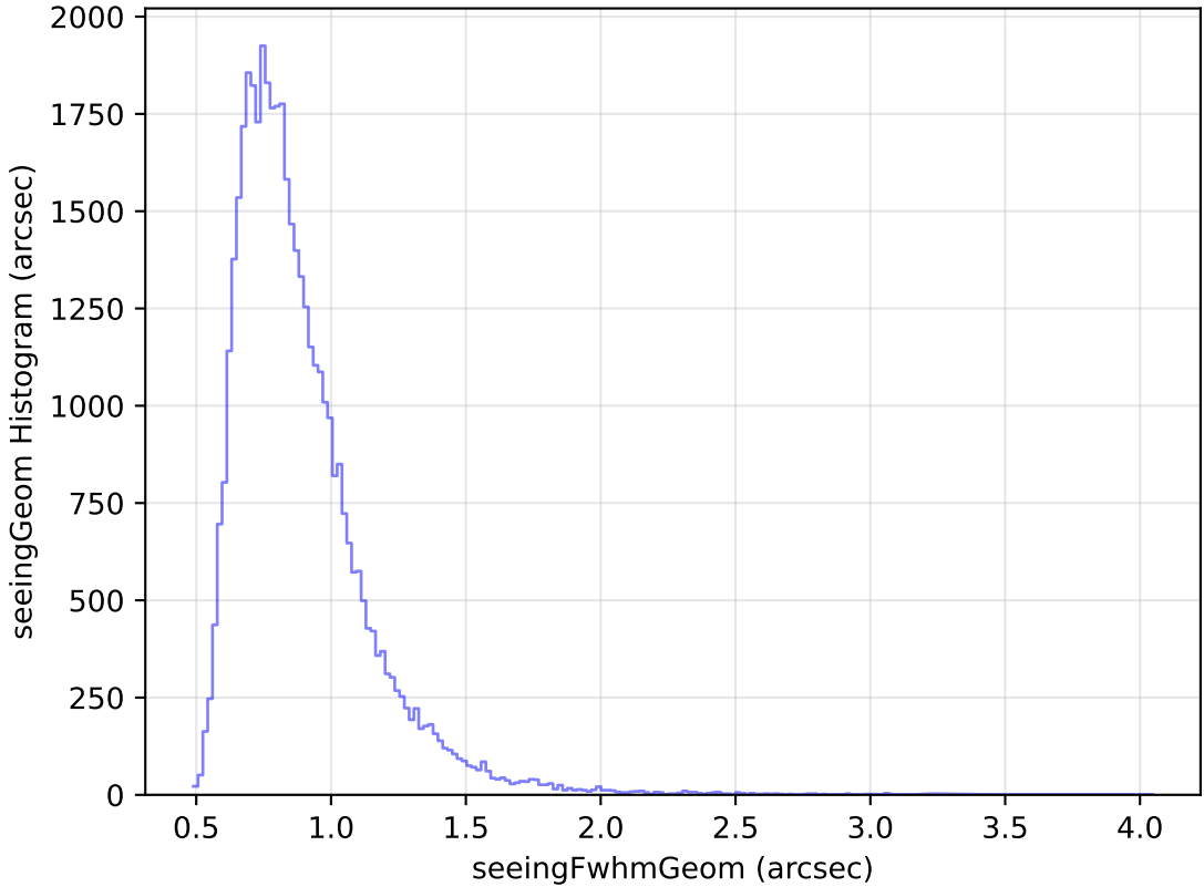
roll_pause_mjdp0_v3.4_10yrs Yr 1 z band: seeingGeom Histogram
