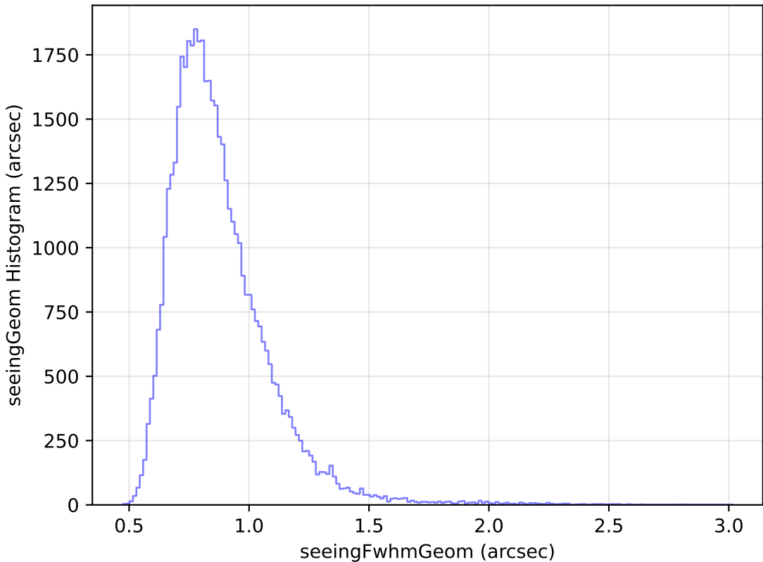
roll_pause_mjdp0_v3.4_10yrs Yr 1 y band: seeingGeom Histogram
