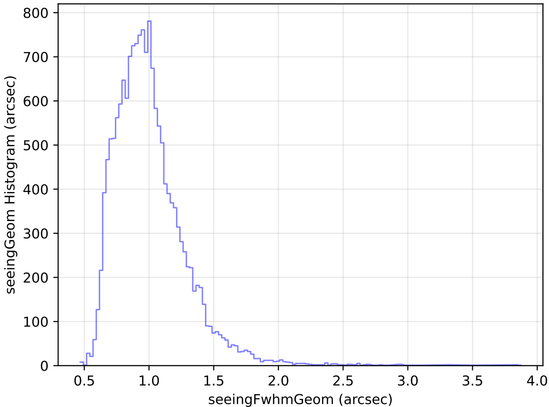
roll_pause_mjdp0_v3.4_10yrs Yr 1 u band: seeingGeom Histogram
