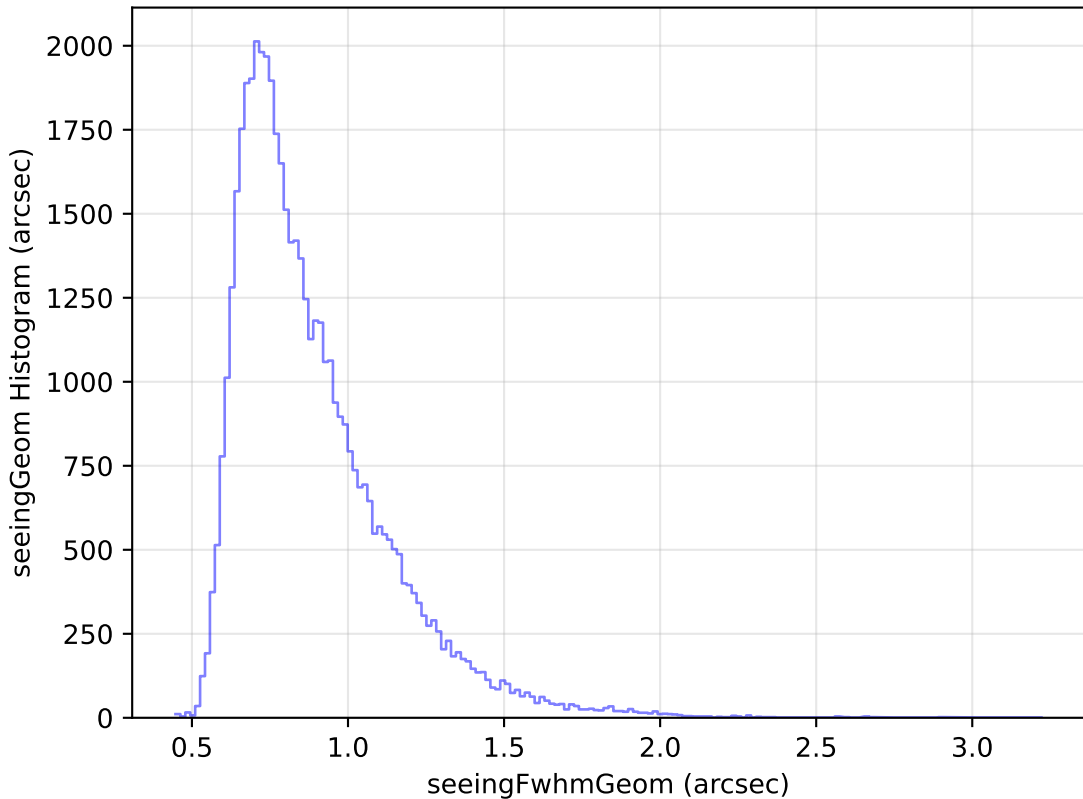
roll_pause_mjdp0_v3.4_10yrs Yr 1 r band: seeingGeom Histogram
